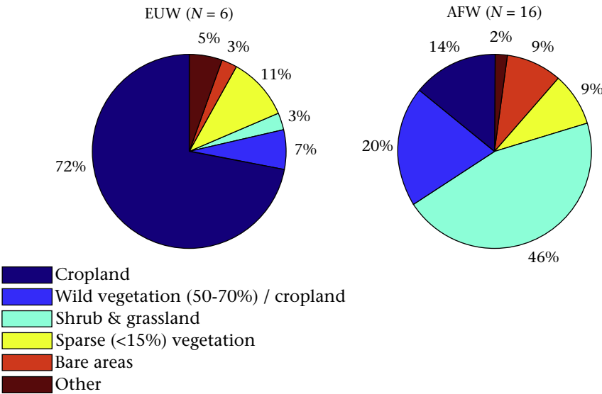
Figure 4. Habitat use of storks wintering in Europe (EUW) versus Africa (AFW). Land use data are based on ESA GlobCover 2009 (© ESA 2010 and UCLouvain, http://due.esrin.esa.int/page_globcover.php ).
